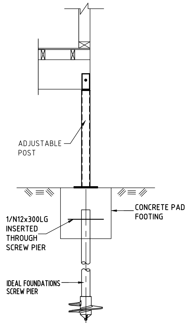
TYPICAL SCREW PIER DETAIL FOR PIERS WITH PAD FOOTING
